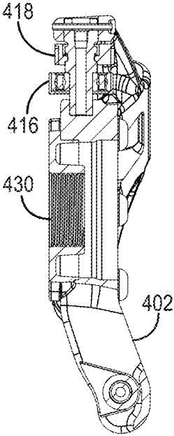
SECTION C-C
