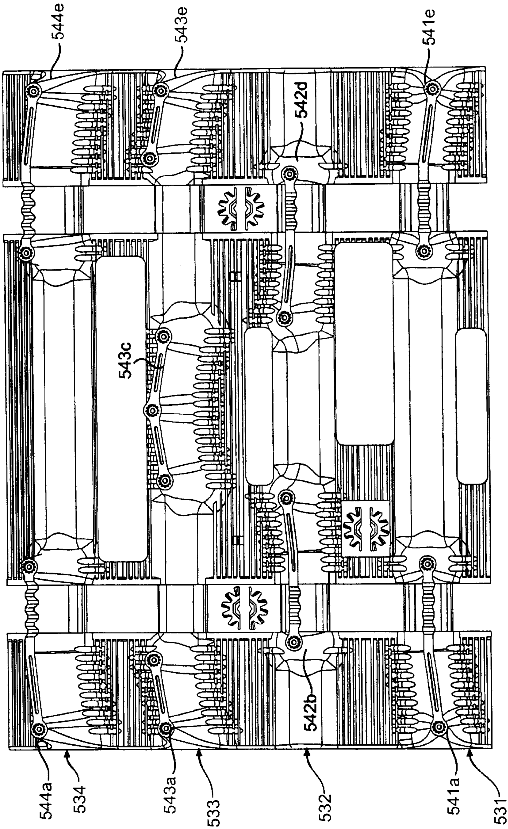
FIG. 11 PRIOR ART
